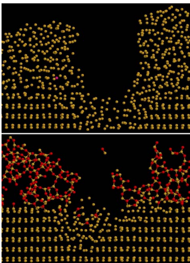
Fig. 3. (Color online) Examples of craters in a-Si/c-Si and a-SiO 2 /c-Si.
